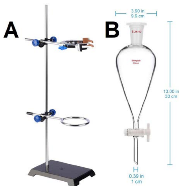
Fig. 1. The stand and the separatory funnel used in this study
