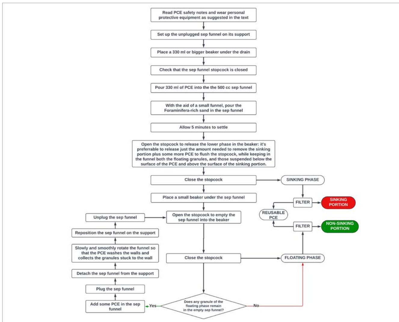
Fig. 4. Density separation with Perchloroethylene – Workflow
