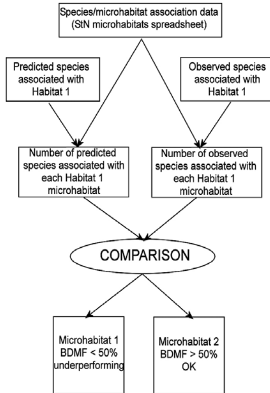
Fig. 3 - Diagrammatic representation of the basic procedure followed in identifying underperforming microhabitats in a macrohabitat (habitat 1) itself recognised as underperforming in maintaining its potential biodiversity. A microhabitat for which less than 50% of the predicted species are observed is taken to be performing its biodiversity maintenance function with less than 50% efficiency. BDMF = biodiversity maintenance function.
